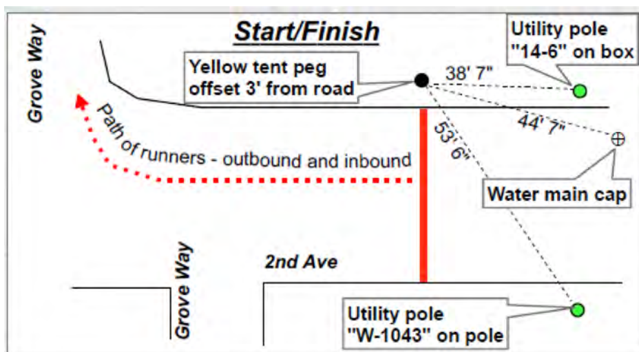
Start/Turnaround/Finish Detail from Cert Map
